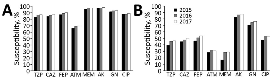
Figure 2. Annual susceptibility rates to antimicrobial agents among imipenem-susceptible (A) and imipenem-resistant (B) Pseudomonas aeruginosa isolates Zhejiang Province, China. AK, amikacin; ATM, aztreonam; CAZ, ceftazidime; CIP, ciprofloxacin; FEP, cefepime; GN, gentamicin; MEM, meropenem; TZP, piperacillin/tazobactam.
