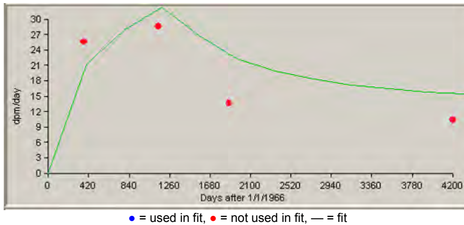
Figure C-29. Predicted 50th-percentile urinary excretion of type M promethium from 1966 to 1979 based on two independent intakes, compared to bioassay data.
