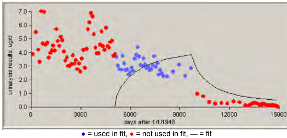
Figure C-22. 50th-percentile uranium urinalysis data for intakes of type S material, 1962 to 1974.
