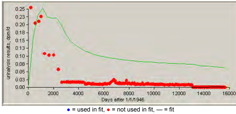
Figure C-11. Predicted 50th-percentile urinary excretion of type M plutonium from 1946 to 1988 based on four independent intakes, compared to bioassay data.
