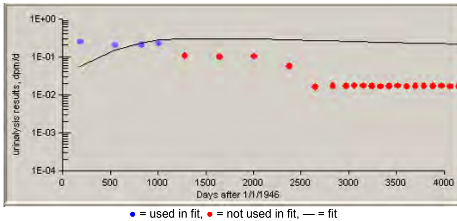
Figure C-12. 50th-percentile plutonium urinalysis data for intakes of type S material, 1946 to 1948.
