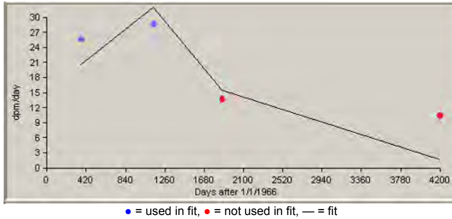
Figure C-30. 50th-percentile promethium urinalysis data for intakes of type S material, 1966 to 1969.
