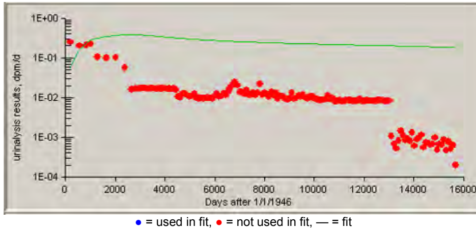
Figure C-16. Predicted 50th-percentile urinary excretion of type S plutonium from 1946 to 1988 based on four independent intakes, compared to bioassay data.
