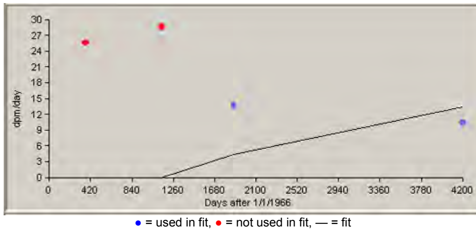
Figure C-31. 50th-percentile promethium urinalysis data for intakes of type S material, 1970 to 1979.
