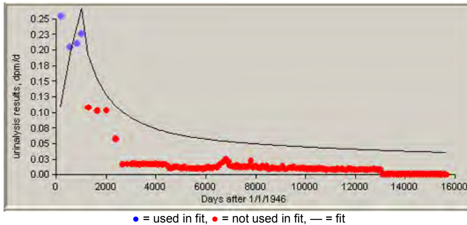
Figure C-7. 50th-percentile plutonium urinalysis data for intakes of type M material, 1946 to 1948.
