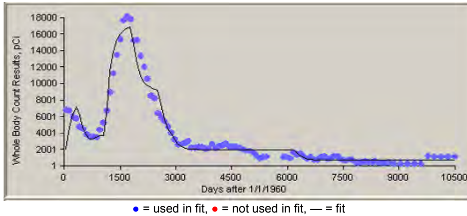
Figure C-43. 50th-percentile 137 Cs whole-body counting data for inhalation intakes of type F material, 1960 to 1988.
