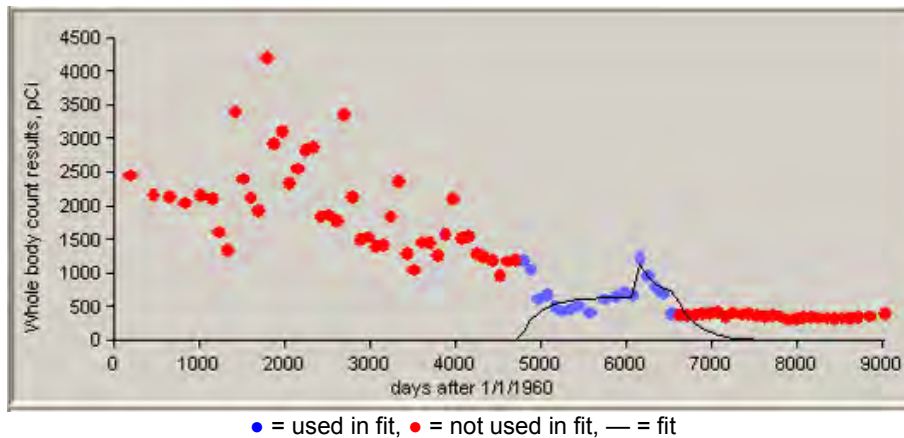
Figure C-37. 50th-percentile zinc whole-body counting data for inhalation intakes of type S material, 1973 to 1977.
