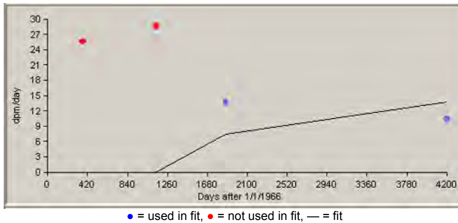
Figure C-28. 50th-percentile promethium urinalysis data for intakes of type M material, 1970 to 1979.
