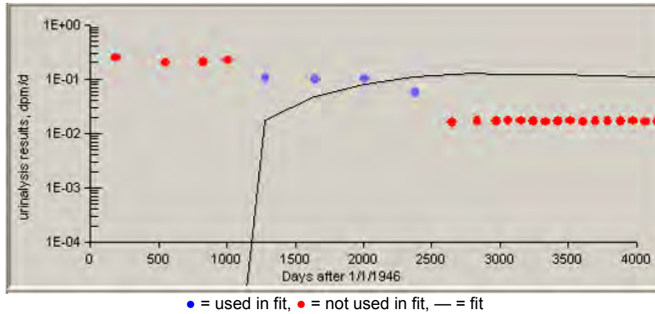
Figure C-13. 50th-percentile plutonium urinalysis data for intakes of type S material, 1949 to 1952.
