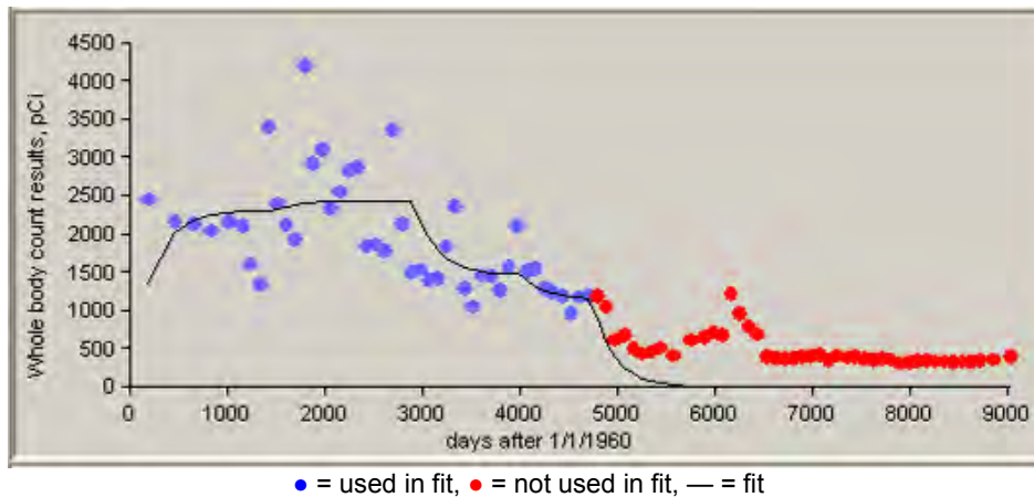
Figure C-40. 50th-percentile zinc whole-body counting data for ingestion intakes, 1960 to 1984.
