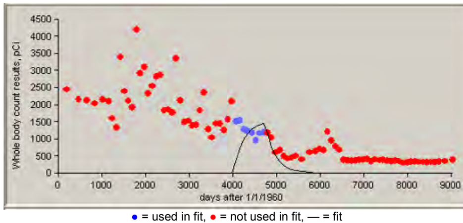
Figure C-36. 50th-percentile zinc whole-body counting data for inhalation intakes of type S material, 1971 to 1972.
