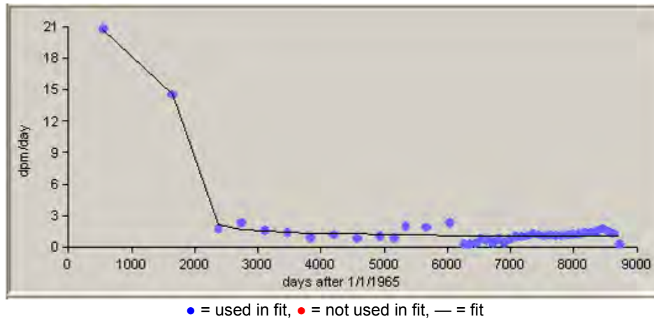
Figure C-26. 50th-percentile strontium urinalysis data for intakes of type F material, 1965 to 1988.
