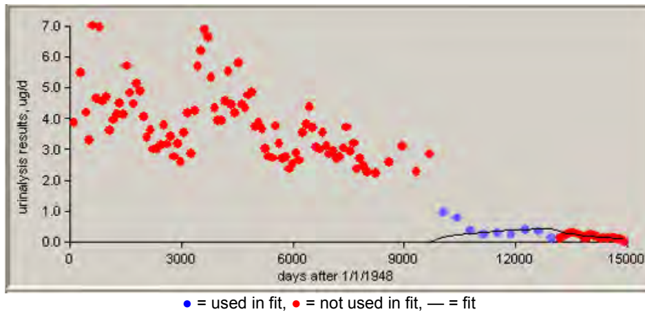
Figure C-23. 50th-percentile uranium urinalysis data for intakes of type S material, 1975 to 1983.
