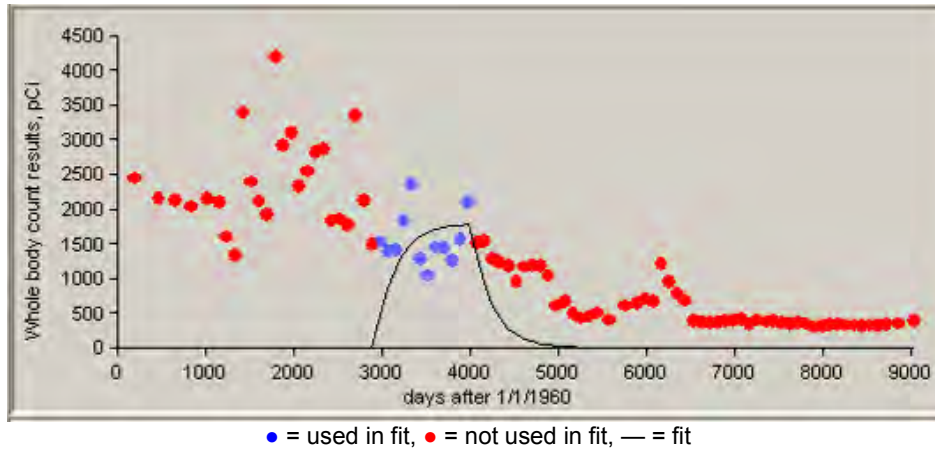
Figure C-35. 50th-percentile zinc whole-body counting data for inhalation intakes of type S material, 1968 to 1970.
