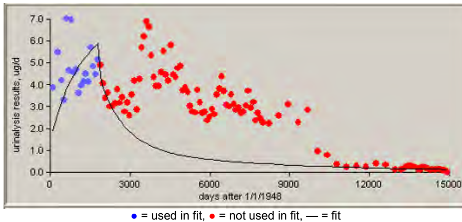
Figure C-19. 50th-percentile uranium urinalysis data for intakes of type S material, 1948 to 1952.
