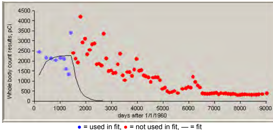
Figure C-33. 50th-percentile zinc whole-body counting data for inhalation intakes of type S material, 1960 to 1963.
