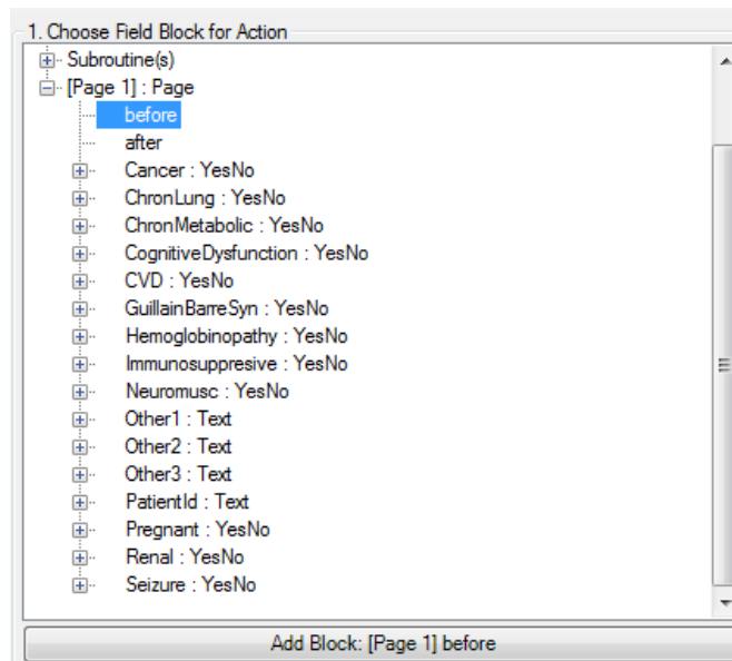
Figure 3.30: Choose Field Block for Action
