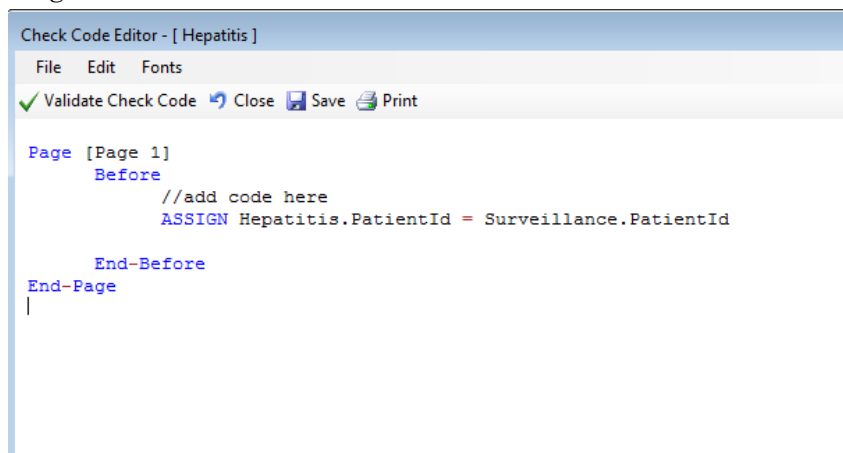
Figure 3.32: Copy Value Check Code Command
