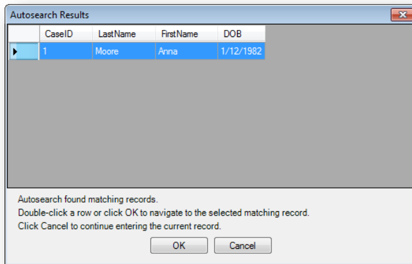
Figure 3.29: Autosearch Results
