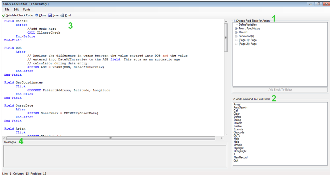
Figure 3.3: Check Code Program Editor
