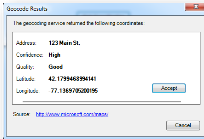
Figure 3.52: Geocode Results
